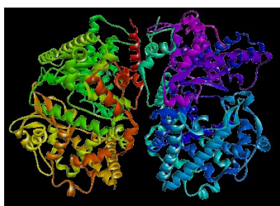
Gambar 1. Reseptor Neprilysin (PDB ID 5jmy)
