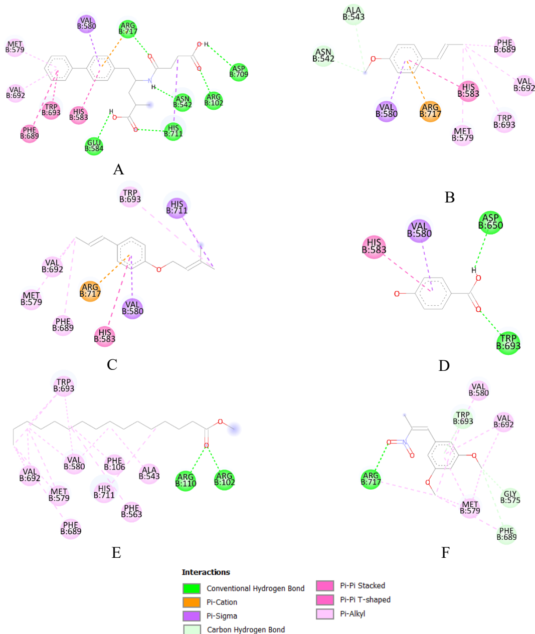
Gambar 3. Interaksi senyawa A (Sacubitrilat), B (Trans anethole), C (1-(3-Methyl-2-butenoxy)-4-(1-propenyl) benzene), D (4-Hydroxybenzoic acid), E (Methyl palmitate), F (3,5-Dimethoxy-β-methyl-β-nitrostyrene) pada reseptor Npyrlisin
